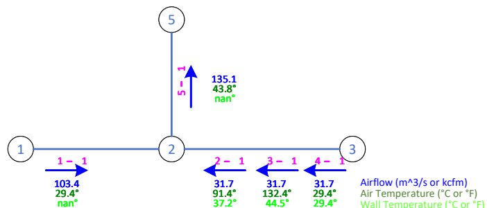
Network Diagram with temperatures
